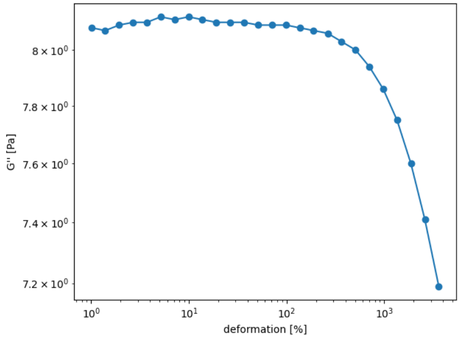
Figure 10: This graph shows the loss module G'' plotted against the deformation of 20%-PVP solution at constant frequency.
